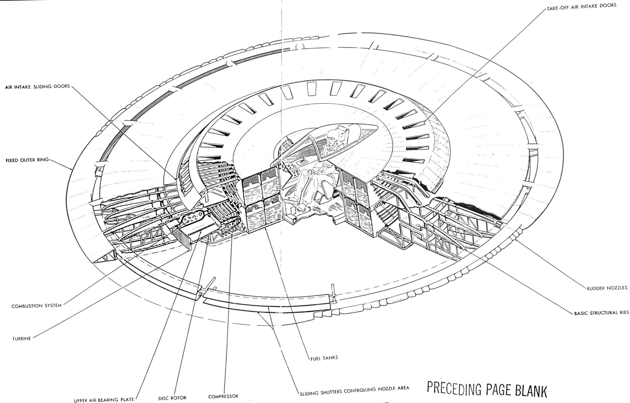
FIG. 2 SECTION CUTAWAY OF RESEARCH AIRCRAFT
