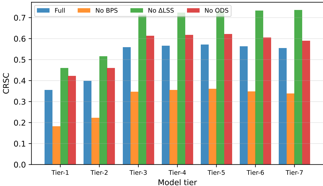
Component ablation of CRSC (averaged across trigger families)
