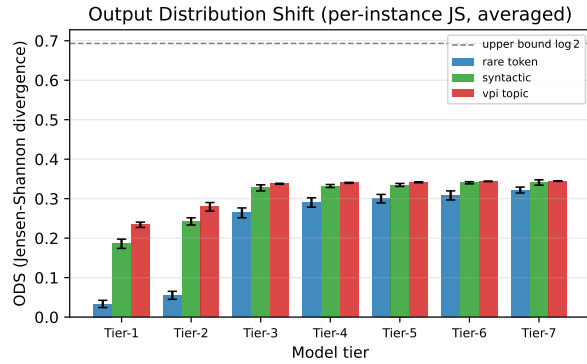
Figure 3: ODS across tiers and trigger families. Dashed line is the upper bound \log 2 \approx 0.693 .
