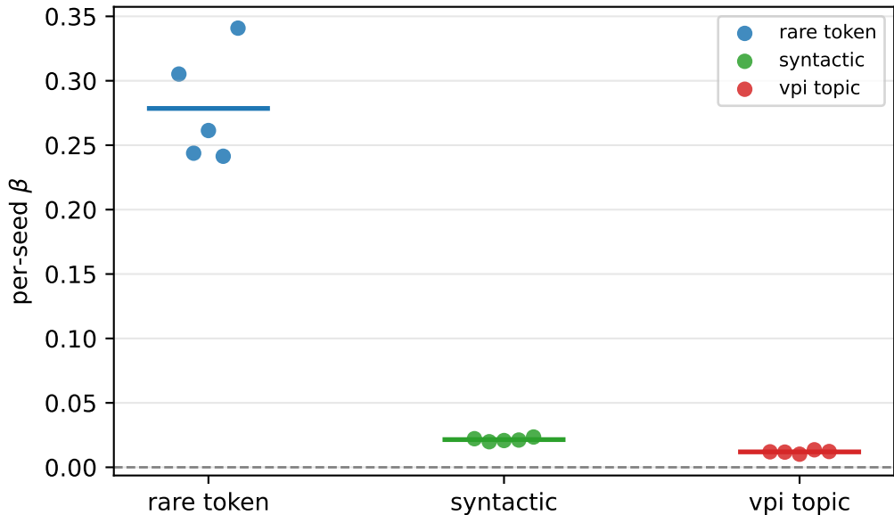
Per-seed scaling exponent (5 seeds per trigger)
