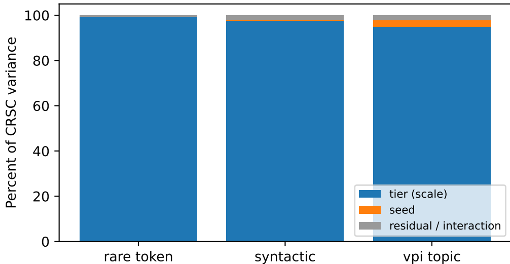
Variance decomposition of CRSC (tier vs seed vs residual)
