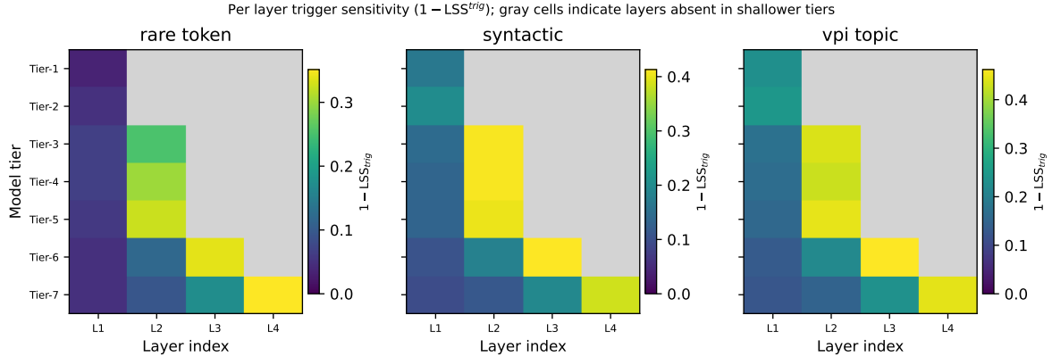
Figure 2: Per layer trigger sensitivity ( 1 - \text{LSS}_l^{\text{trig}} ) by tier and trigger family. Brighter is more sensitive. Gray cells indicate layers absent in shallower tiers.
