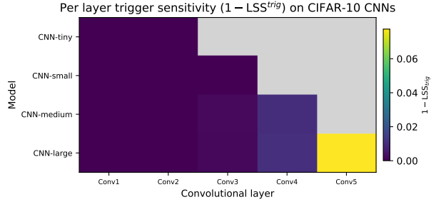
Figure 8: Per convolutional layer trigger sensitivity on the CIFAR-10 CNNs.
