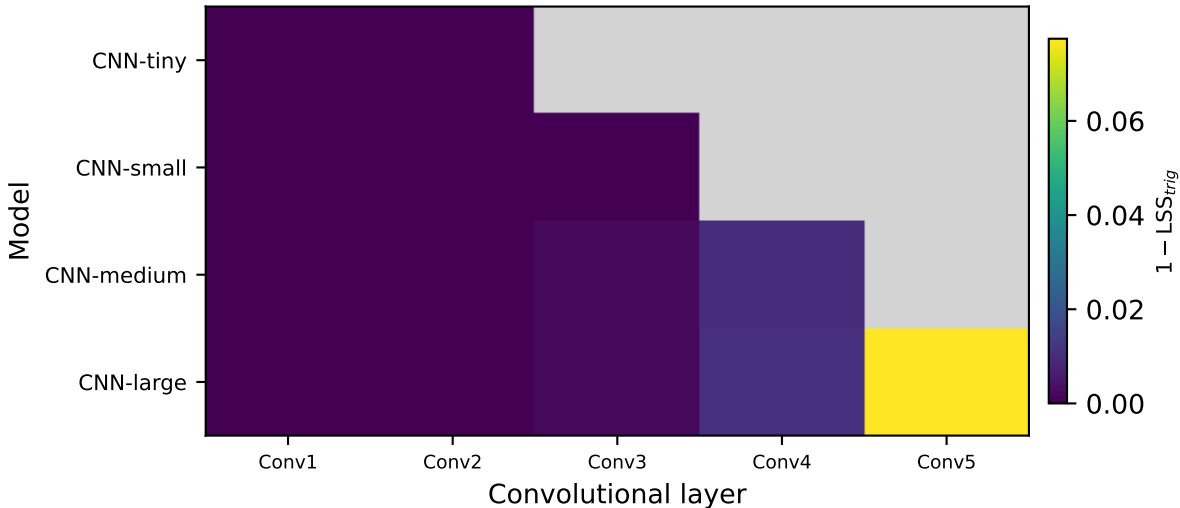
Per layer trigger sensitivity ( 1 - \text{LSS}^{trig} ) on CIFAR-10 CNNs
