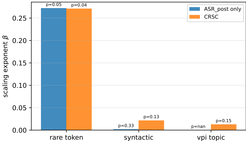
ASR-only vs CRSC scaling exponents (with raw p values)
