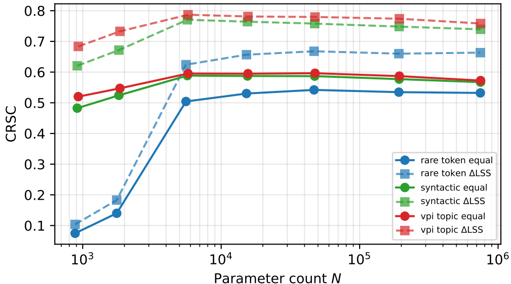
CRSC with \Delta LSS (ratio-normalized) vs equal-weighted
