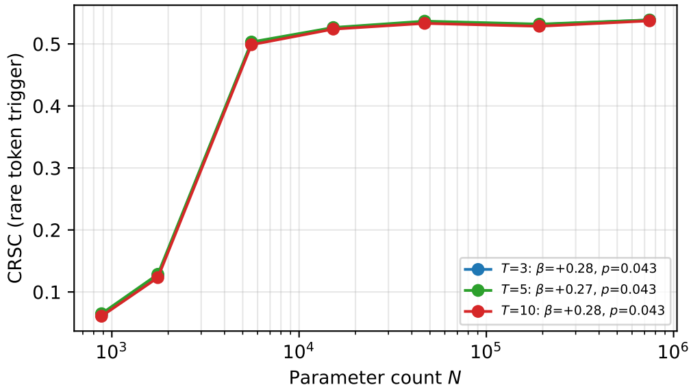
BPS / CRSC sensitivity to number of safety checkpoints T
