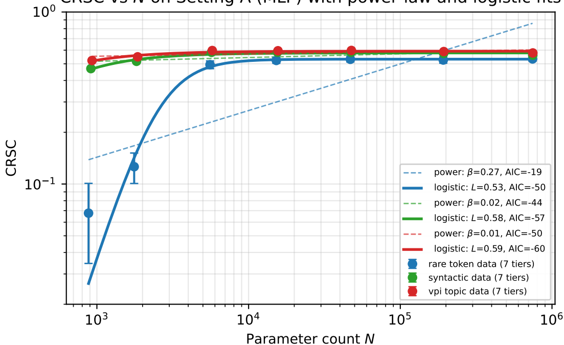
CRSC vs N on Setting A (MLP) with power-law and logistic fits
