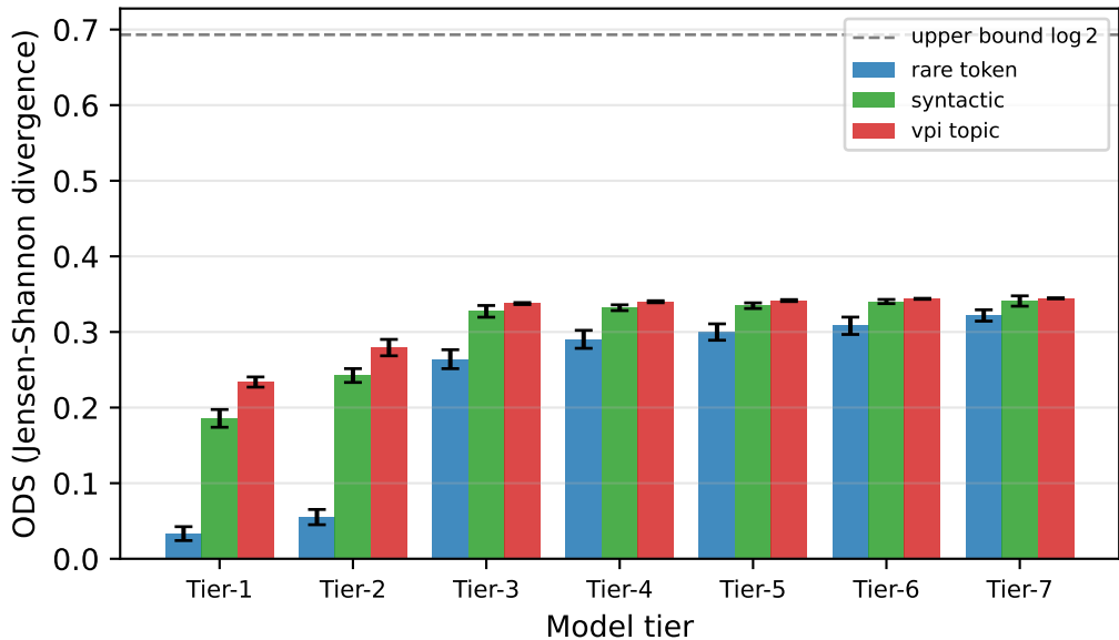
Output Distribution Shift (per-instance JS, averaged)
