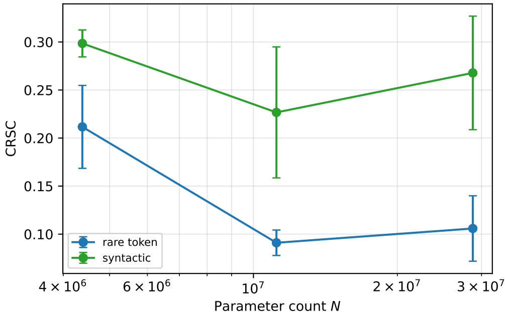
CRSC across pretrained transformers (SST-2)
