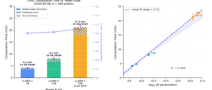
Fig. 5. CRSC computation time vs. model scale on A100-80 GB ( K = 500 probes). Left : stacked bars decompose runtime into hidden-state extraction (dark) and Frobenius norm (light); dashed line tracks the theoretical O(L \cdot K \cdot d) complexity (right axis, normalized to 7B). Annotations show wall-clock time and VRAM footprint per model. Right : log-linear scaling confirms near-linear growth in \log_{10}(N) ( R^2 = 0.998 , slope = 17.3 min/decade). Error bars: \pm 1\sigma over 5 runs.
