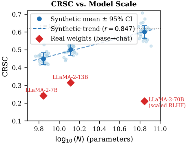
Fig. 3. CRSC vs. model scale ( \log_{10}(N) ). Error bars show 95% bootstrap confidence intervals. All three fine-tuning conditions ( p = 0.01 ) shown. Pearson r = 0.847 , p < 10^{-5} .
