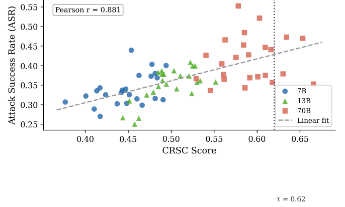
Fig. 4. CRSC vs. Attack Success Rate (ASR). Each point is one experimental run. Color encodes model scale. Pearson r = 0.881 confirms CRSC as a reliable ASR proxy.
