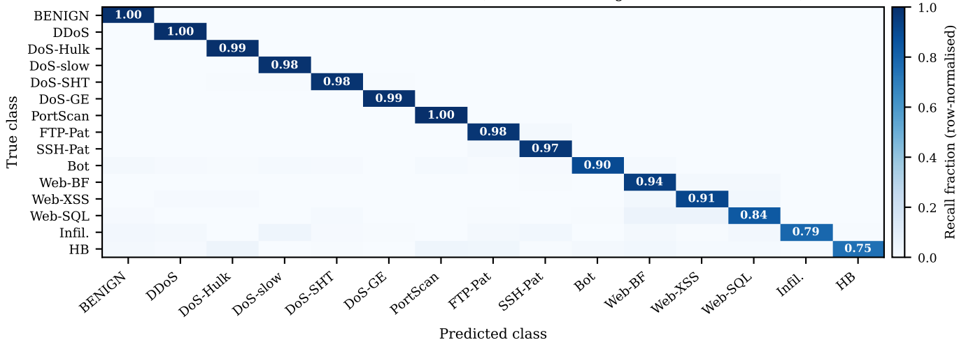
E2 -- Row-normalised confusion matrix (SHIELD-AI surrogate, n=15,000 , seed 42)
