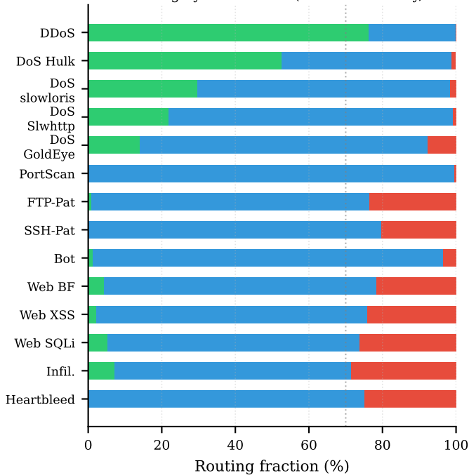
E4 -- PC3 routing by attack class (attack flows only, seed 42)
