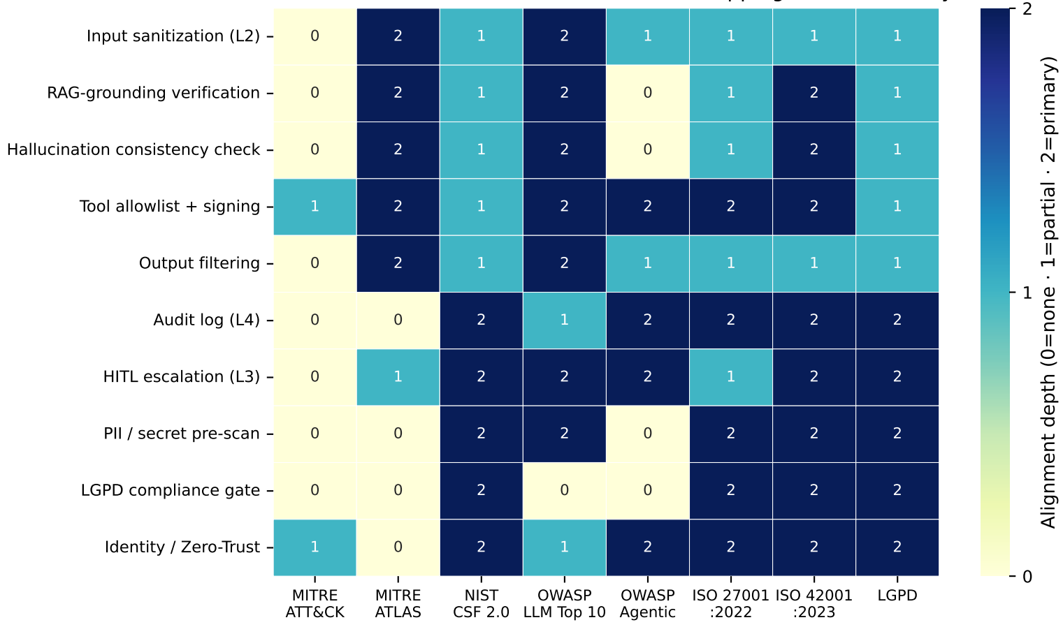
F7 · SHIELD-AI control × external-standard mapping (Table 4 density)
