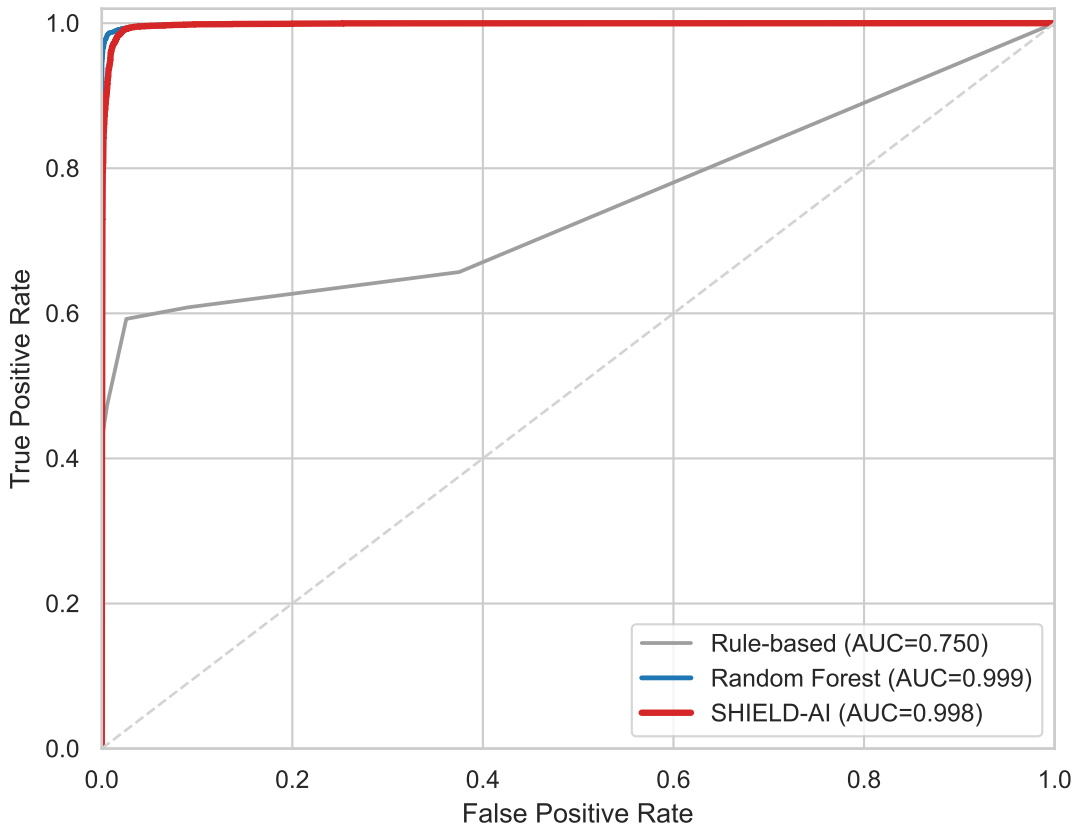
Figure E1: Detection ROC on CICIDS-2017-like data
