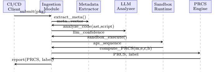
Fig. 2: LLM-Sentry single-package analysis sequence.
