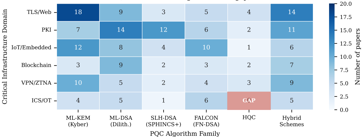
Fig. 2 — Literature Coverage Heatmap: Domain vs. PQC Algorithm (Red = zero coverage / research gap)
