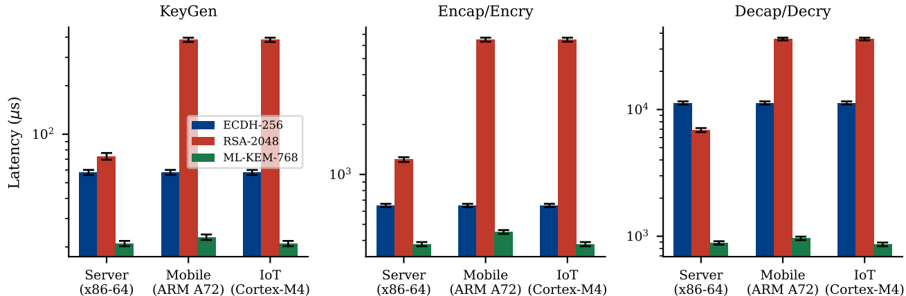
Fig. 3 — Performance: ML-KEM-768 vs ECDH-256 vs RSA-2048 (log scale; mean \pm 1 SD from pqm4/OQS-BoringSSL benchmarks)
