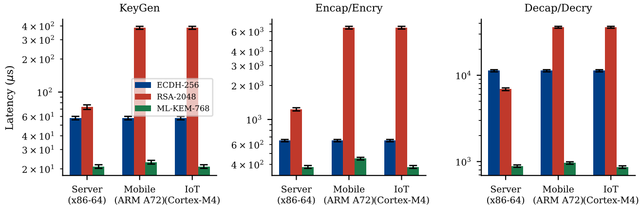
Fig. 3 — Performance Comparison: ML-KEM-768 vs ECDH-256 vs RSA-2048 (Server, Mobile, IoT; log scale; bars = mean \pm 1 SD, n=1000 )
