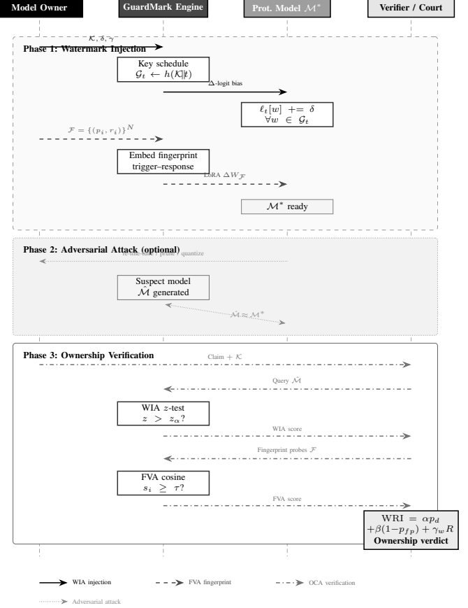
Fig. 2. GuardMark protocol sequence (three phases). Solid: WIA injection; dashed: FVA fingerprint; dash-dot: OCA verification; dotted: attack.
