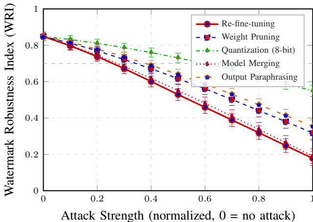
Fig. 4. WRI vs. attack strength, 5 scenarios, 95% CI, 50 trials, seed=42. Dashed: ownership threshold \tau = 0.70 .
