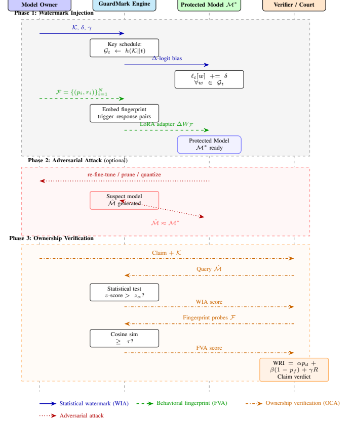
Fig. 2. GuardMark protocol sequence. Blue: WIA token watermarking; green: FVA fingerprint embedding; orange: OCA verification; red: adversarial attack path.
