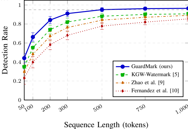
Fig. 3. Detection rate vs. sequence length, 95% CI, 30 trials, \alpha = 0.01 , seed=42.
