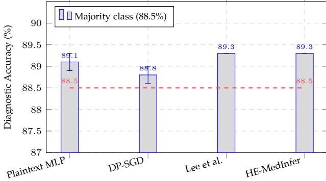
Fig. 3. Accuracy under plaintext and encrypted inference (measured; Table 5). HE-MEDINFER and the Lee et al. proxy are statistically indistinguishable (89.3% each); the majority-class baseline is 88.5% (dashed reference), so accuracy differences compress and AUROC in Table 5 is the primary metric. Plaintext and DP-SGD error bars are 95% CIs over 10 independently trained models; HE-MEDINFER and Lee et al. are single-run point estimates (Sec. 6). Results are computed on the synthetic cohort of Section 6.1, not on MIMIC-III records.
