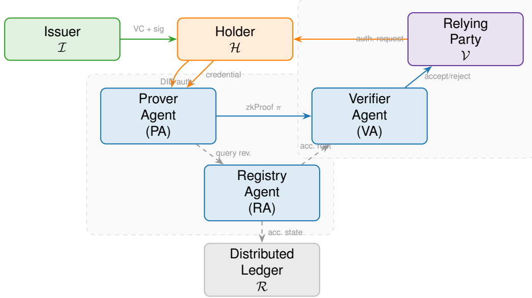
Fig. 1. ZKAuth Framework Architecture. The Prover Agent generates Groth16 zk-SNARK proofs over Poseidon-hashed credential attributes. The Verifier Agent performs constant-time pairing-based proof verification. The Registry Agent maintains DID Documents and a sparse Merkle tree accumulator for credential revocation. All inter-agent communication is authenticated with the holder's DID-bound key pair. Arrows indicate data flow; dashed arrows denote on-chain operations.
