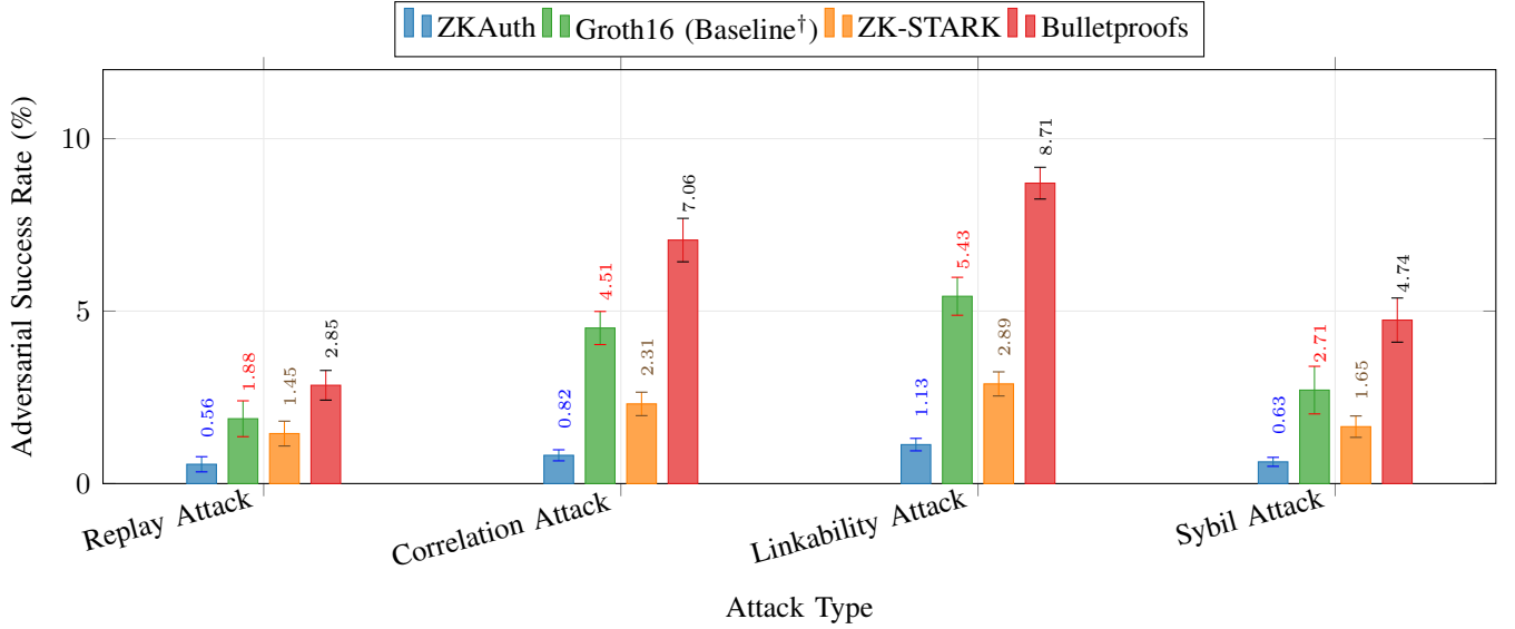
Fig. 5. Adversarial success rate (%) per attack vector and authentication scheme. Lower bars indicate stronger resistance. Error bars represent 95% confidence intervals (10 simulation runs per cell). ZKAuth achieves the lowest success rate across all four attack types. Data are simulation-based. Attack definitions follow Table II.
