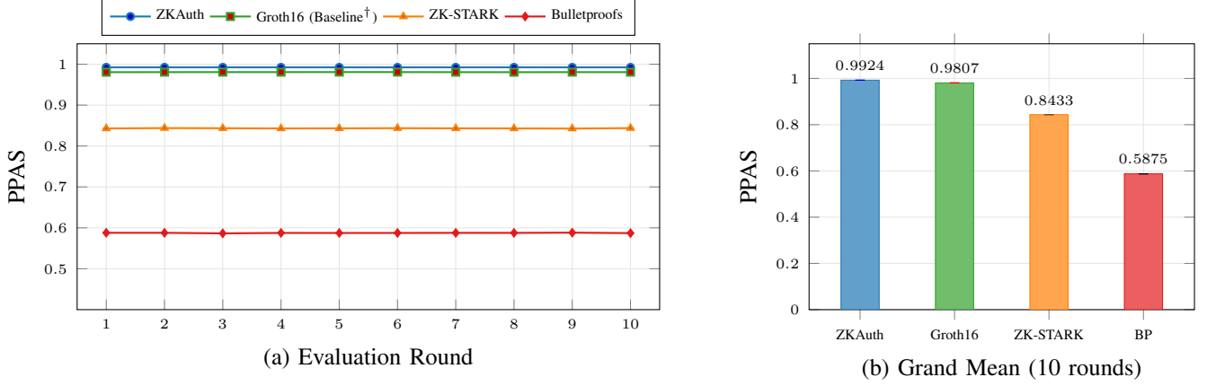
Fig. 4. Privacy-Preserving Authentication Score (PPAS) for all schemes: (a) per-round trajectories across the 10 evaluation rounds; (b) grand mean over the 10 rounds with 95% confidence intervals (values annotated above each bar; CIs are smaller than the marker size at this scale). ZKAuth achieves the highest PPAS ( 0.9924 \pm 0.0001 ), significantly outperforming all baselines ( p < 0.001 ). Data are simulation-based; ground-truth PPAS parameters follow Definition 3.
