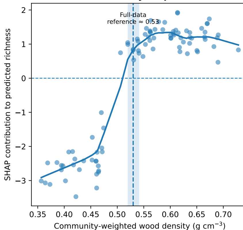
B CWM wood-density response
