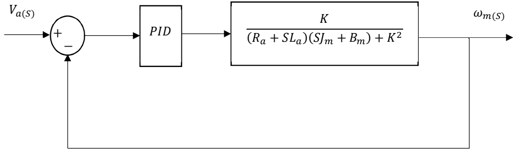
Fig. 3.3: Block Diagram of the Closed Loop Model
