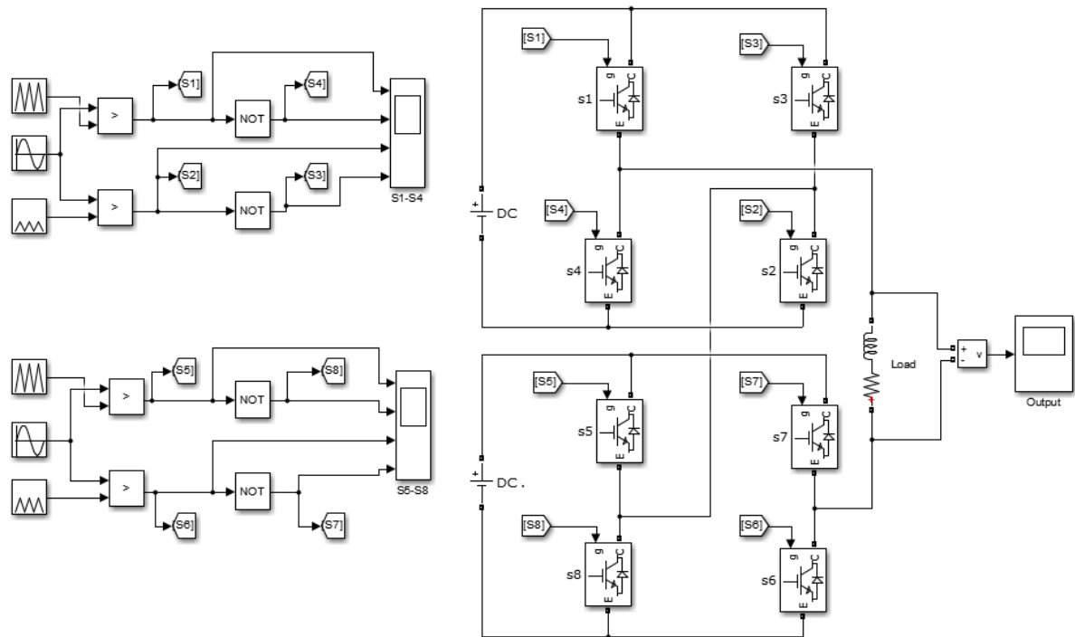
Fig. 3.8: Overall model of the system
