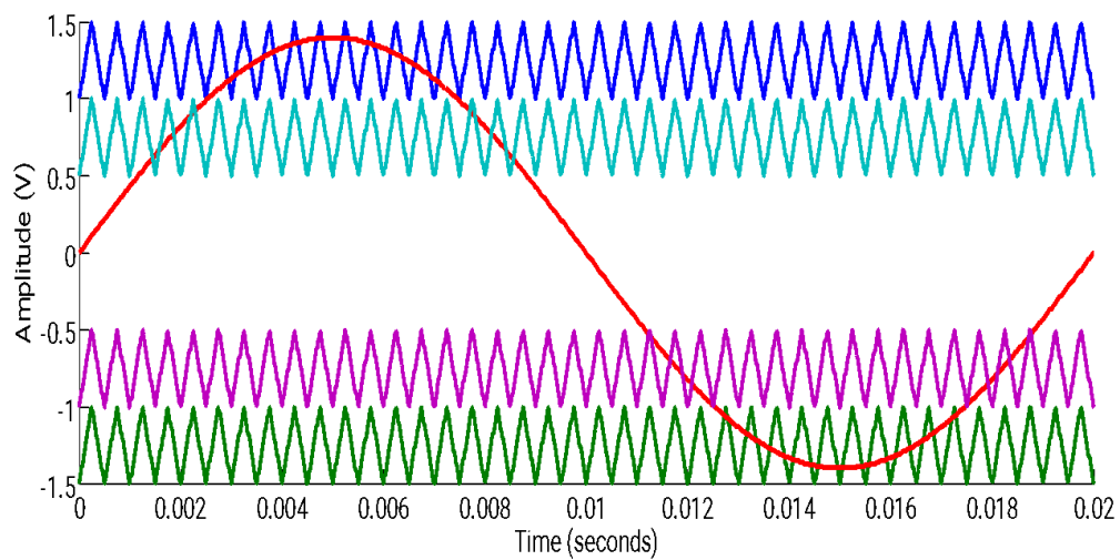
Fig. 4.5: Overall Signal Modulation
