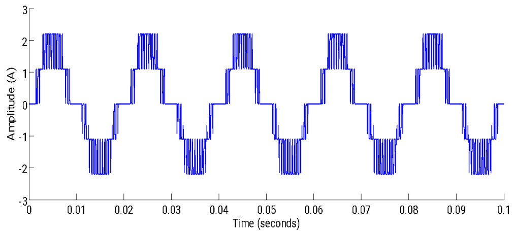
Fig. 4.8: Output current with R-L load
