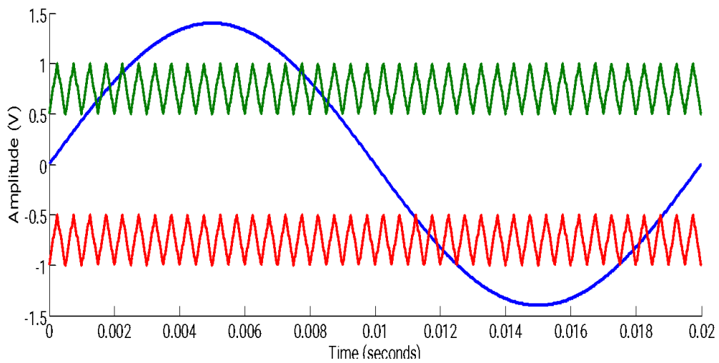
Fig. 4.4: Comparing sine and triangular for S5 - S8
