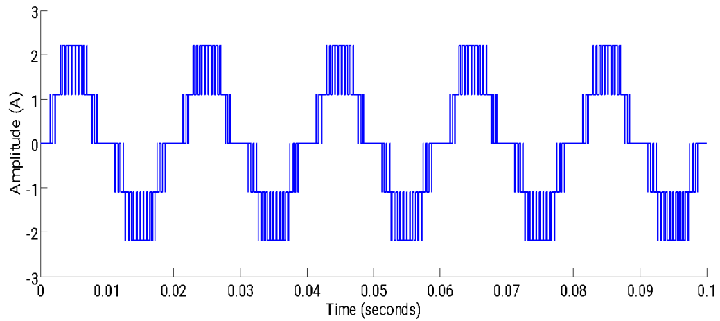
Fig. 4.7: Output current with a resistive load
