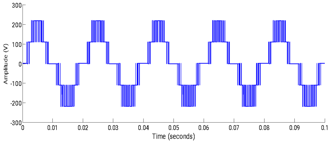
Fig. 4.6: Output voltage
