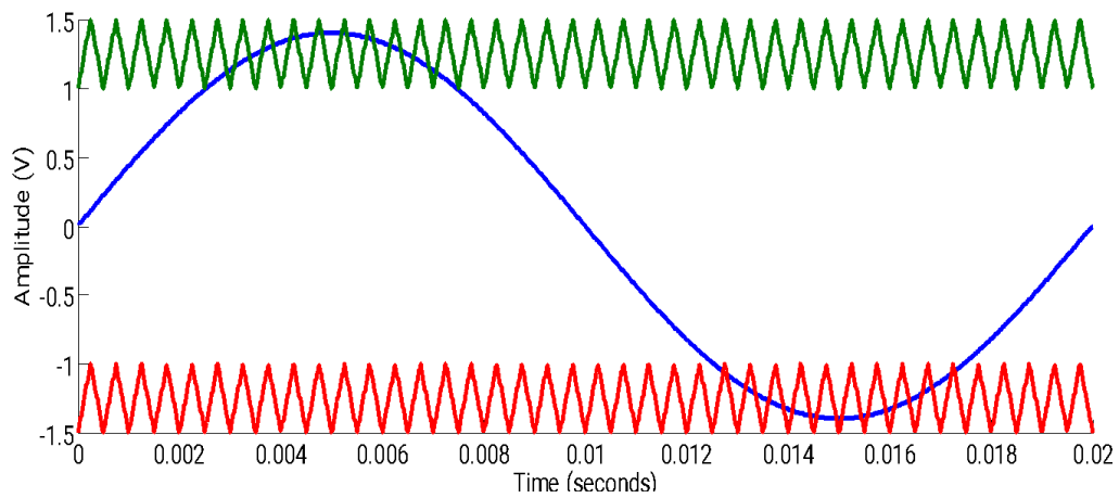
Fig. 4.3: Comparing sine and triangular for S1 - S4
