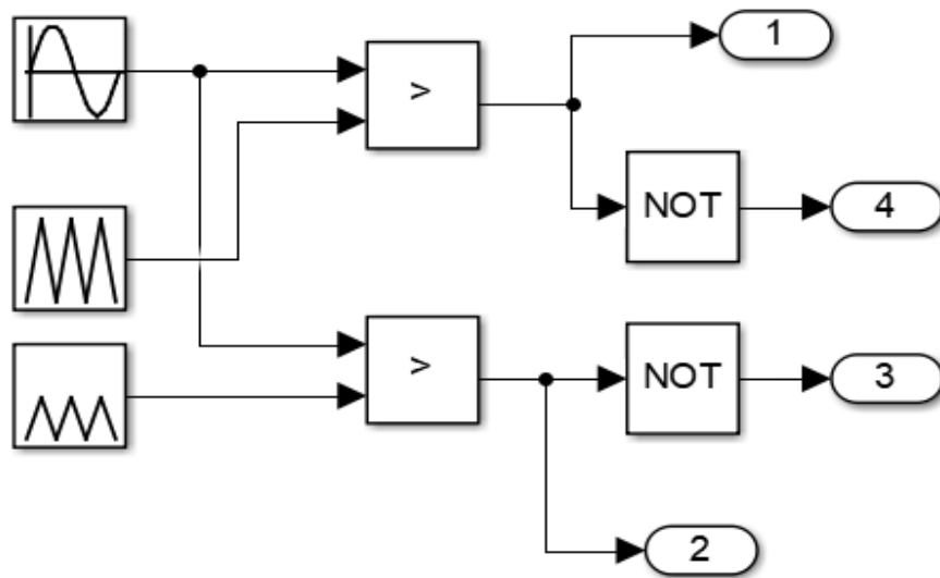
Fig. 3.6: SPWM switching pulses for switches S1 - S4
