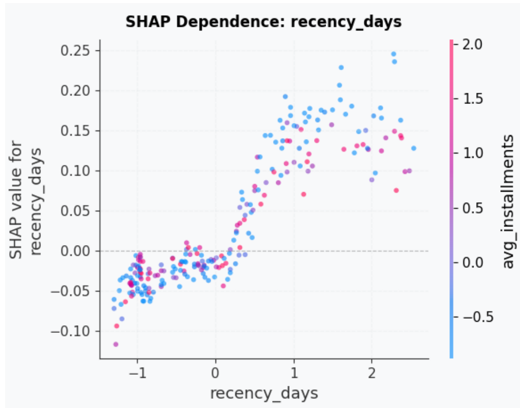
Figura 16 – Dependence plots da feature recency_days no SHAP (Random Forest)
