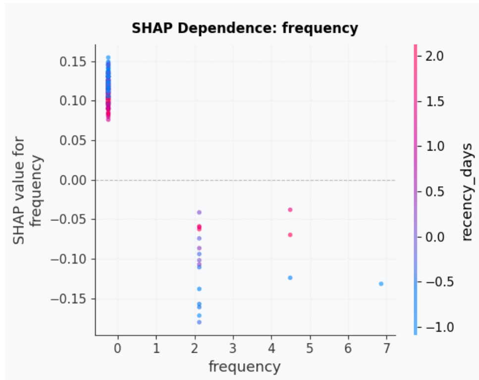
Figura 15 – Dependence plots da feature frequency no SHAP (Random Forest)
