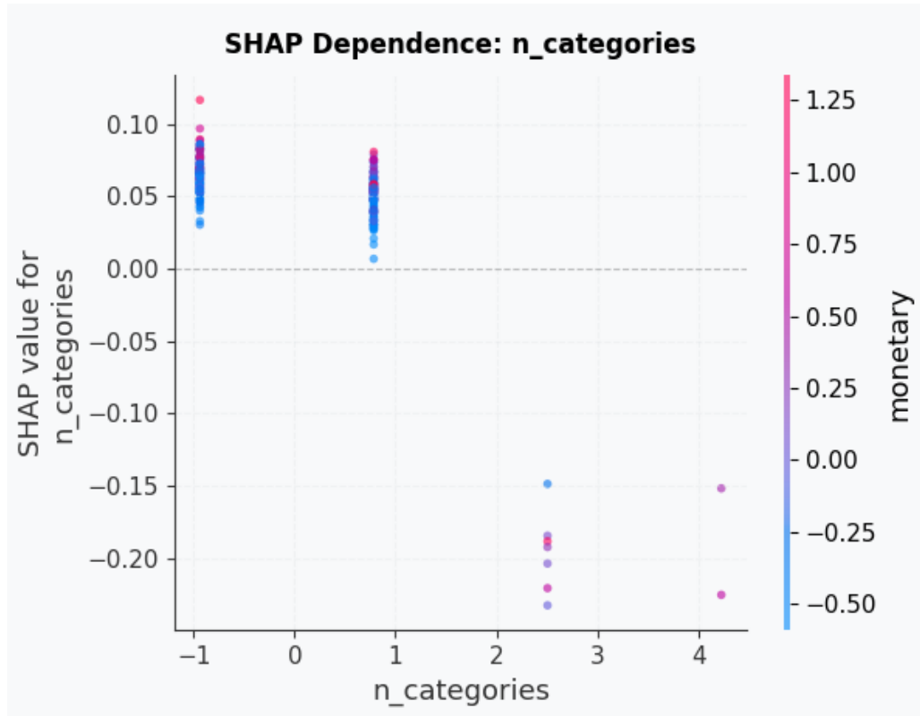
Figura 17 – Dependence plots da feature n_categories no SHAP (Random Forest)
