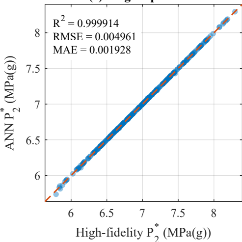
(c) Stage-2 pressure
