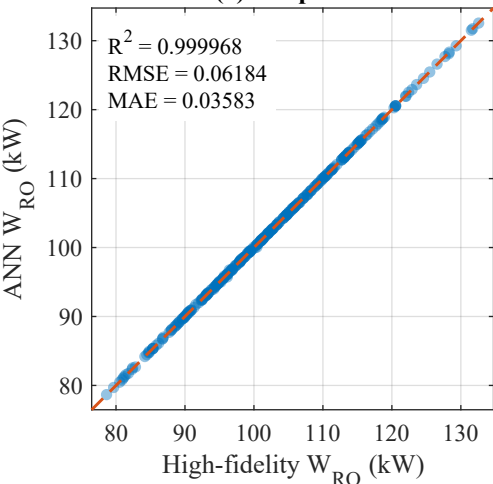
(a) RO power
