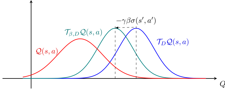
Figure 1: Evolution of the Pessimistic Distributional Bellman Backup. While \mathcal{T}_D^\pi \mathcal{Q}(s, a) is overestimated, a corrected backup \mathcal{T}_{\beta, D}^\pi \mathcal{Q}(s, a) is closer to \mathcal{Q}(s, a) .
