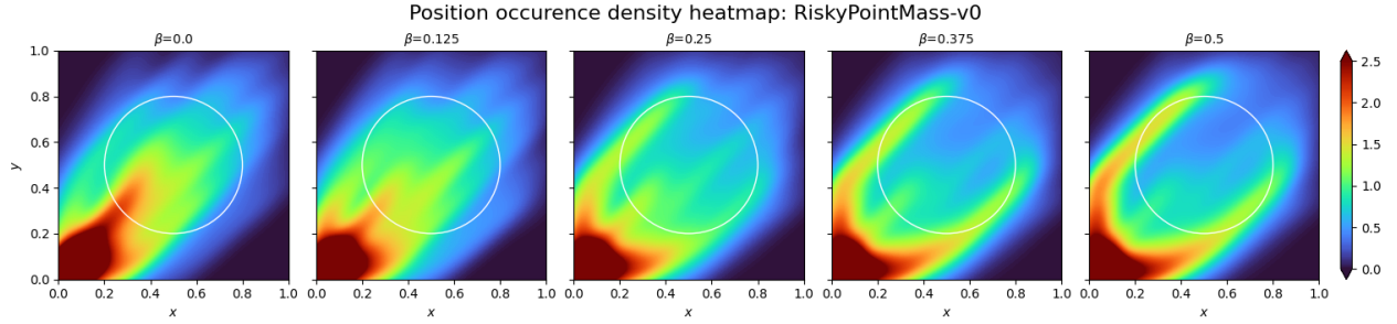
Figure 4: Position occurrence density heatmap of STAC on RiskyPointMass-v0 for different \beta values. The white circle represents danger zone.
