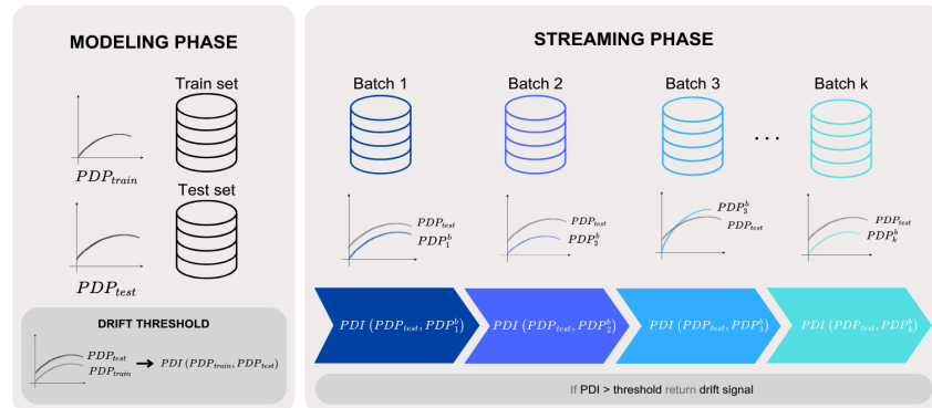
Figure 2: The workflow of the Profile Drift Detection
