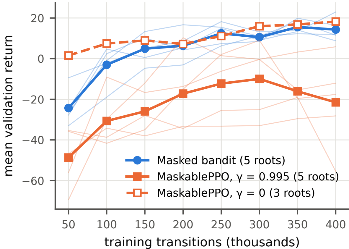
Figure 6.1: Mean validation return (seeds 2001–2005) during training. Thin lines: individual roots. PPO with \gamma = 0.995 is unstable across roots; with \gamma = 0 it learns as fast as the bandit.
