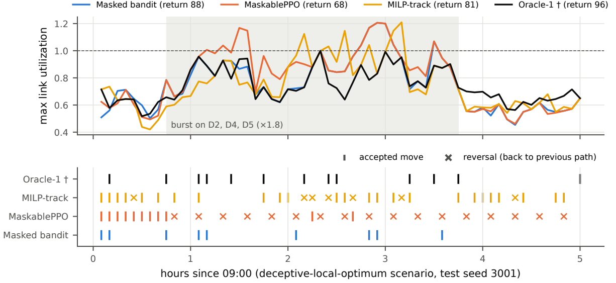
Figure 6.3: One test episode (deceptive-local-optimum, seed 3001; learners of root 314159). Top: worst link utilization; bottom: accepted moves ( \times = return to the previous path within six intervals). PPO flips one demand every three intervals, the hold-down period; the bandit makes few moves. Oracle-1 sees the next interval’s traffic and is shown for reference.
