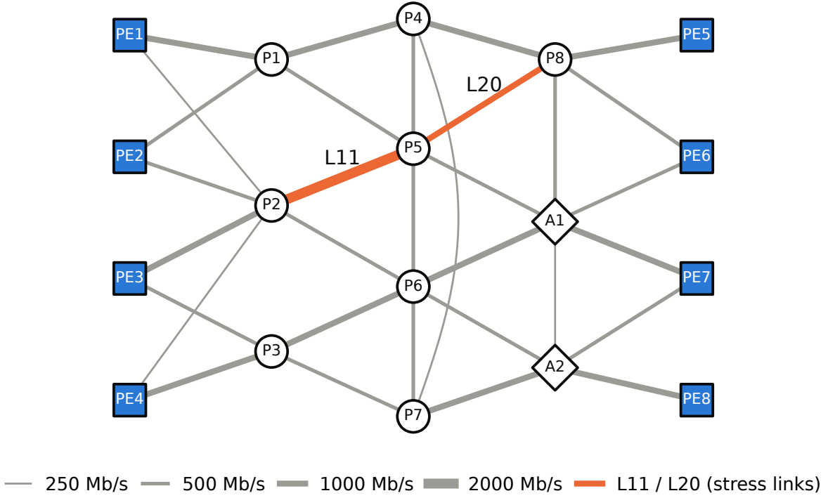
Figure 3.1: Backbone topology: 4 ingress and 4 egress PE routers (squares), 8 core (circles) and 2 aggregation routers (diamonds); line width encodes per-direction capacity. L11 and L20 are the links whose failure or saturation the scripted scenarios stress.
