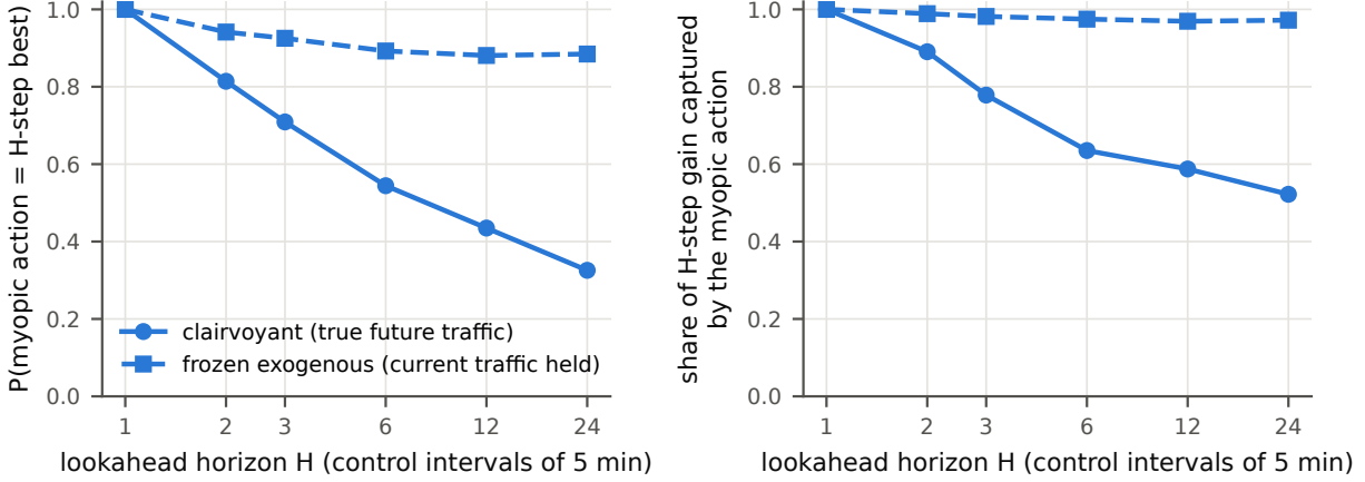
Figure 6.2: Open-loop sequentiality diagnostic (greedy-visited states; from 495 states at H = 1 to 390 at H = 24 , since states near an episode’s end lack H remaining intervals). Left: probability that the action with the best first-interval reward is also the best over H intervals (“take it, then change nothing”). Right: share of the best H -interval gain that the myopic action captures. Solid: rollouts carry the episode’s true future traffic and failures (clairvoyant). Dashed: traffic and link state held at their current values.
