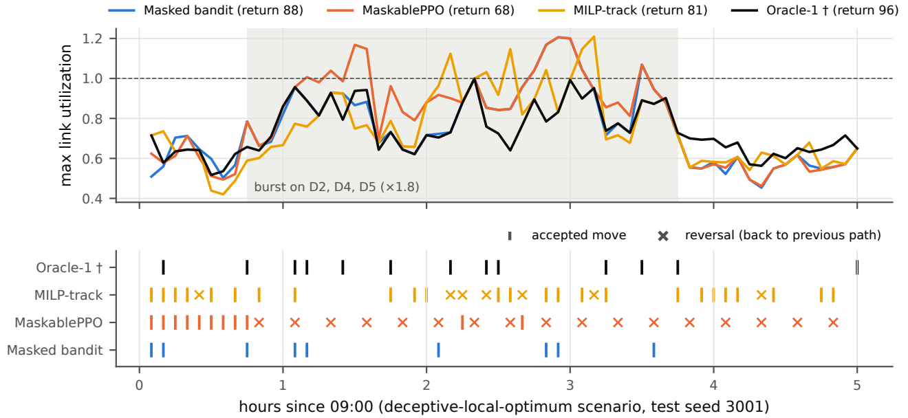
Figure 2: One test episode (deceptive-local-optimum, seed 3001; learners of root 314159). Top: worst link utilization; bottom: accepted moves ( \times = return to the previous path within six intervals). PPO flips one demand every three intervals, the hold-down period; the bandit makes few moves. Oracle-1 sees the next interval’s traffic and is shown for reference.
