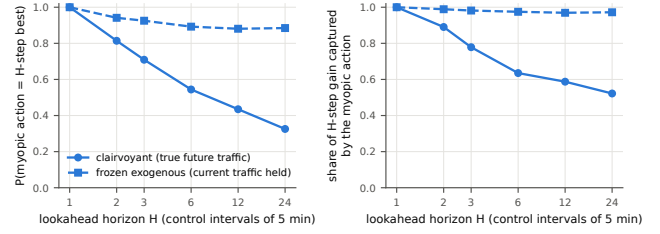
Figure 1: Sequentiality diagnostic on 390 paired states. Left: probability that the action with the best first-interval reward is also the best over H intervals (“take it, then change nothing”). Right: share of the best H -interval gain that the myopic action captures. Solid: rollouts carry the episode’s true future traffic and failures (clairvoyant). Dashed: traffic and link state held at their current values.
