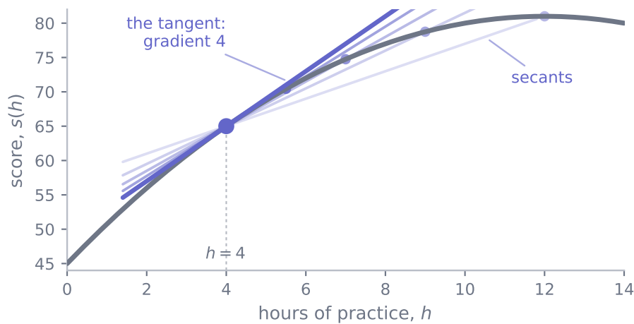
Figure 1: Each faint line joins h = 4 to a point further along the curve; its gradient is one row of the table above. As that second point slides in, the lines settle onto the single bold line — the tangent, whose gradient is 4.
