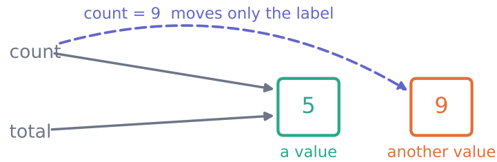
Figure 1: Assignment attaches a name to a value. Two names can label the same value; reassigning one moves that label without touching the value or the other name.
