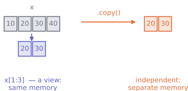
Figure 1: A basic slice is a view — a second way of looking at the same memory, so writing through it changes the original. Advanced indexing, and .copy() , produce independent data.
