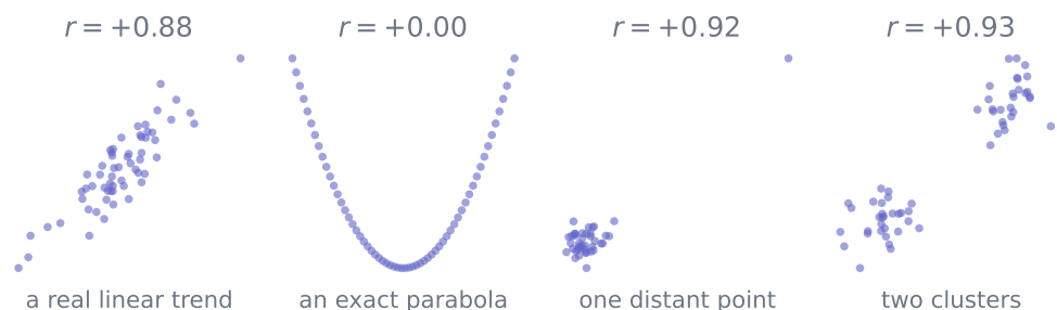
Figure 2: Four datasets. Three have correlations near +0.9 and nothing else in common; the fourth has a correlation of exactly zero and a perfect relationship — every y is determined by its x . One number cannot certify a shape.
