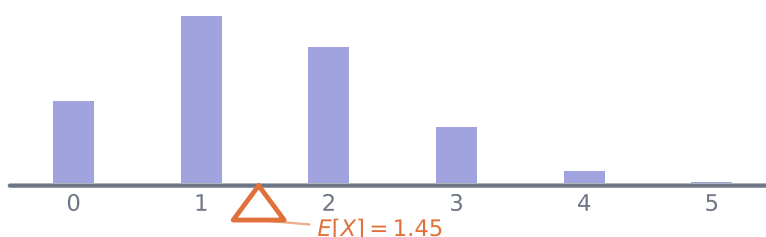
Figure 2: The left-hand distribution from the previous figure, treated as a pile of weights on a plank. The expected value is the point where it balances — which is why an expectation, unlike a median, is dragged about by values far from the centre.
