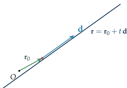
Figure 5: A line as a point \mathbf{r}_0 plus all multiples of a direction \mathbf{d} .
