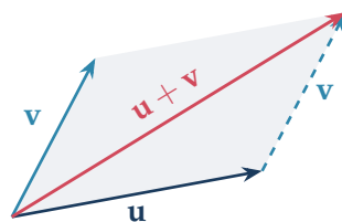
Figure 1: The triangle (and parallelogram) rule for \mathbf{u} + \mathbf{v} .
