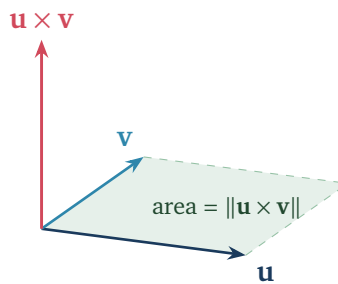
Figure 4: \mathbf{u} \times \mathbf{v} is perpendicular to the plane of \mathbf{u}, \mathbf{v} ; its length is the parallelogram's area. (Schematic: \mathbf{u} \times \mathbf{v} points out of the plane of \mathbf{u}, \mathbf{v} , not within the page.)
