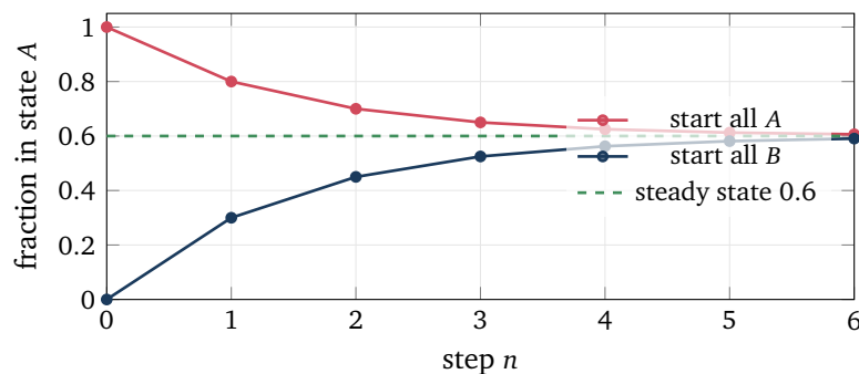
Figure 3: Two very different starts both converge to the steady state 0.6, at the rate set by the second eigenvalue 0.5.
