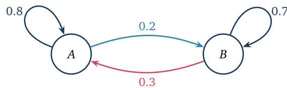
Figure 2: The two-state chain: arrows carry the one-step transition probabilities, and the probabilities leaving each state sum to one.
