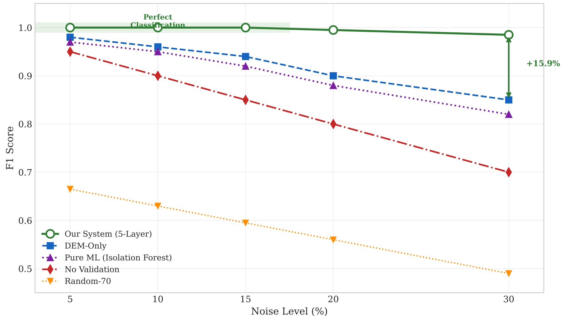
Validation Performance vs. Noise Level
