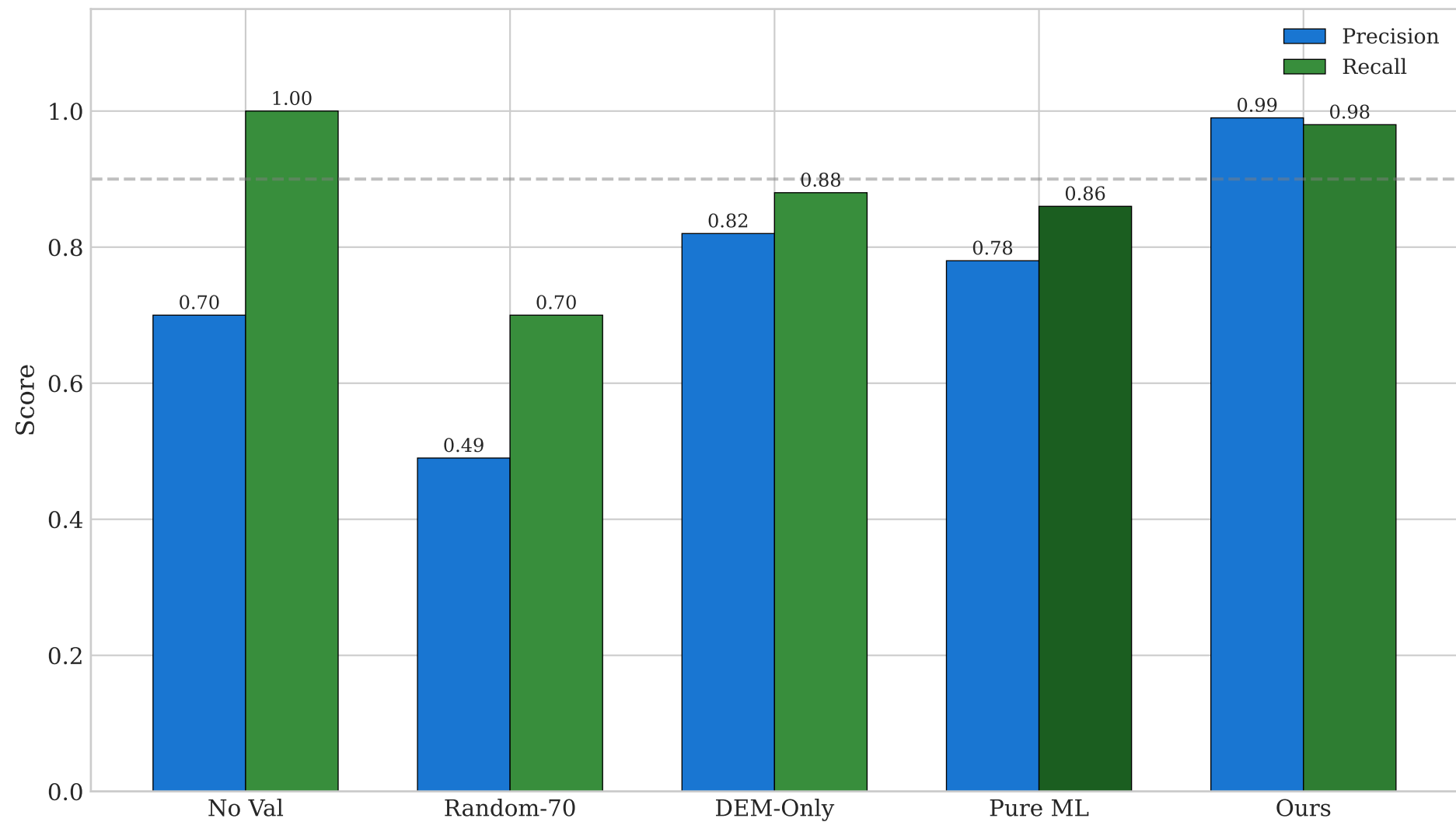
Precision and Recall at 30% Noise Level
