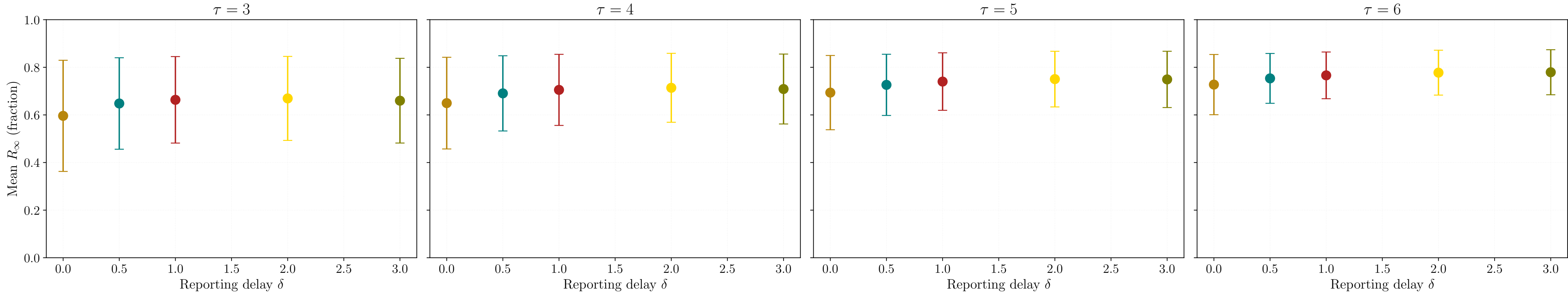
Effect of Intervention Delay on Final Epidemic Size
